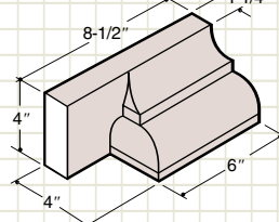
W14-R-ST-LT (SHOWN) W14-R-ST-RT
